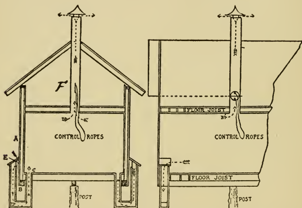
Sketch D—Showing the Rutlerford System of Ventilation. (Hoard's Dairyman.)
